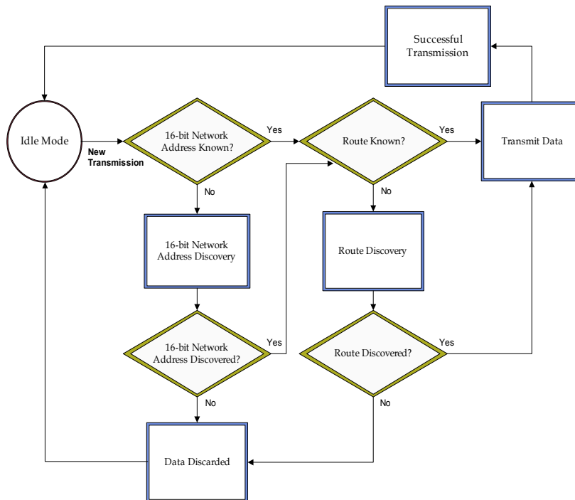
Figure 2-04. Transmit Mode Sequence
