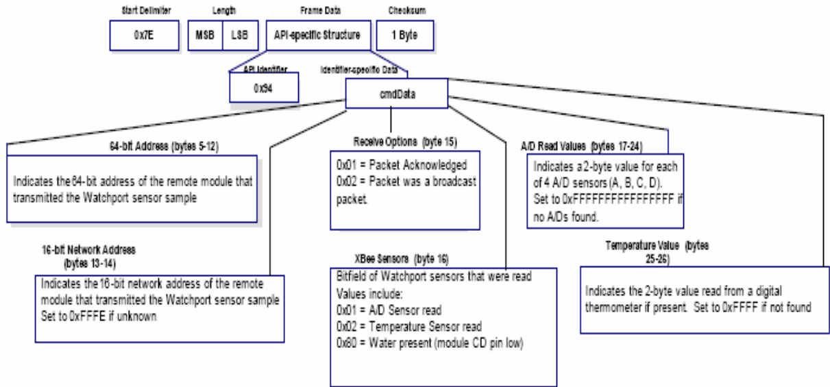
Figure 7-18. XBee Sensor Read Indicator (0x94)
