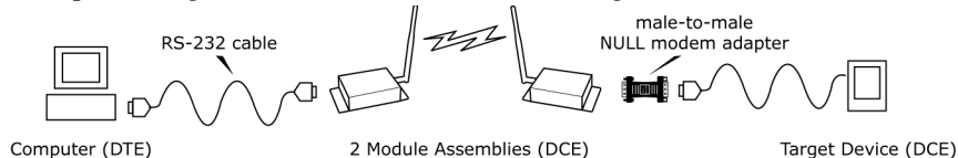
Figure B-08. Example of a Digi Radio Modem (DCE node) connecting to another DCE node
