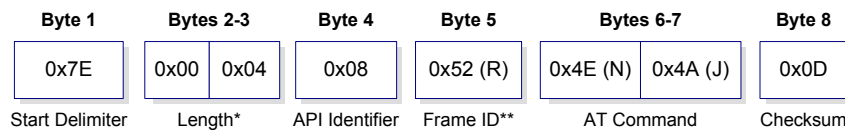
Figure 7-7. Example: API frames when reading the NJ parameter value of the module.
